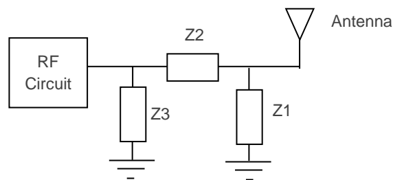
Figure 2 – PI matching network example
