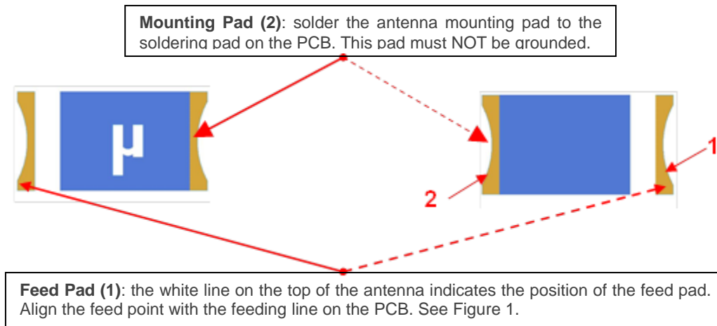
Figure 6 – Pads of the Fractus Micro Reach Xtend™ chip antenna.
