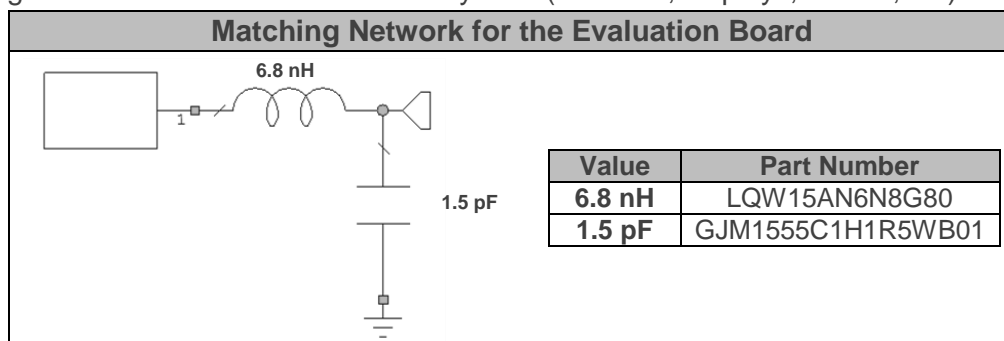
Figure 5 – Matching network implemented in the evaluation Board.
