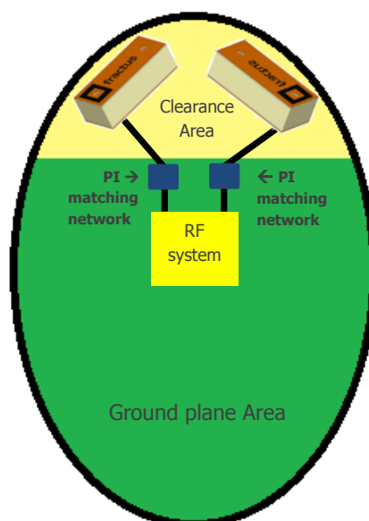
Example 4. MIMO with two FR05-S1-NO-1-004 antennas
