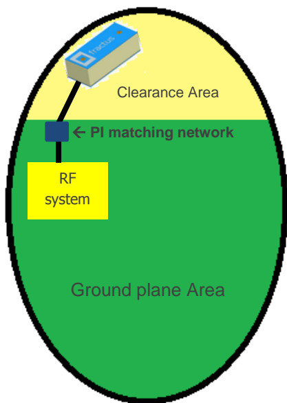
Example 1. With one FR05-S1-N-0-102 antenna
