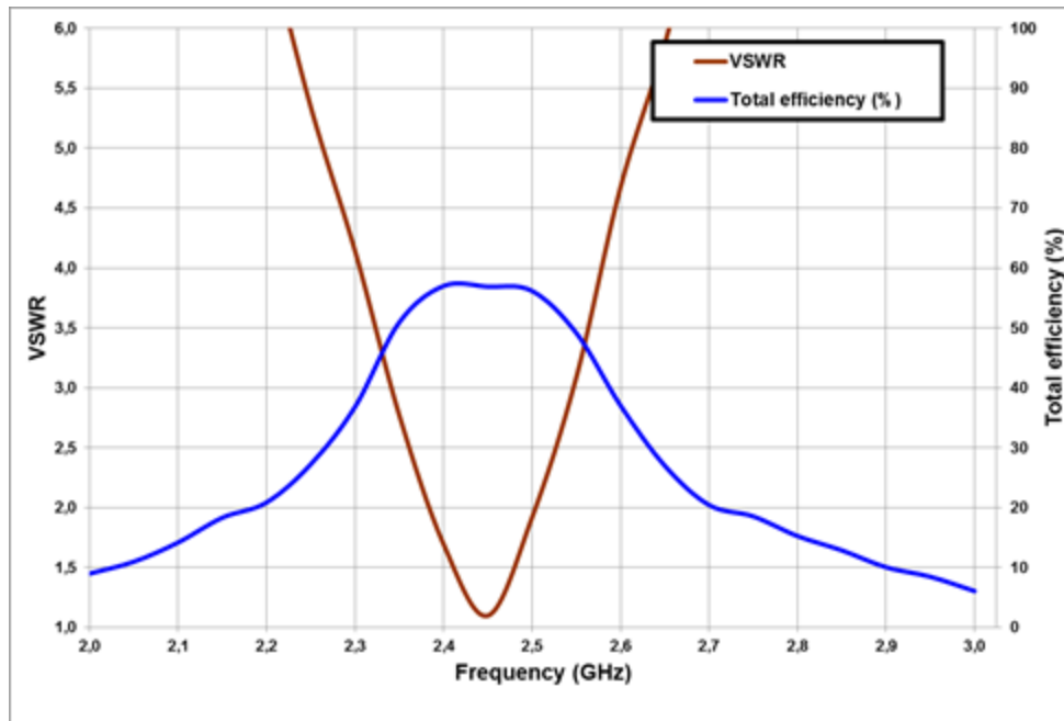
Figure 2 – VSWR (Voltage Standing Wave Ratio) and Efficiency (%) vs. Frequency.
