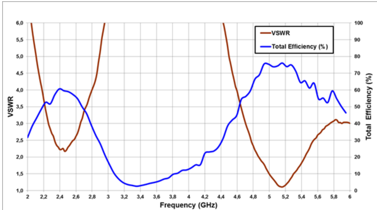
Figure 3 – VSWR (Voltage Standing Wave Ratio) and Total Efficiency (%) vs. Frequency.
