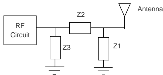
Figure 2 – PI matching network example
