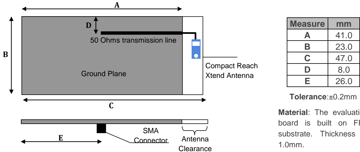
Figure 1 – EB_FR05-S1-N-0-102. Compact Reach Xtend™ Evaluation Board.
