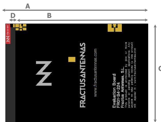
Figure 4 – EB_FR01-S4-224-CR80-1561-1606 in CR80 standard format. Evaluation Board providing operation for BeiDou E1 band (1561 MHz), GPS L1 band (1575 MHz) and for GLONASS L1 band (from 1598 MHz to 1606 MHz).
