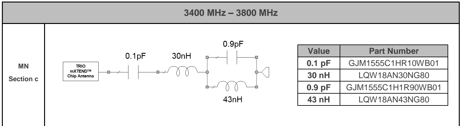
Figure 4 – Matching network implemented in the Evaluation Board port #2 (Figure 1).
